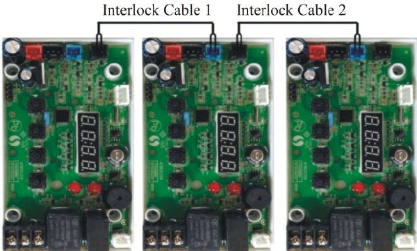
Figure 3-9 Interlock
