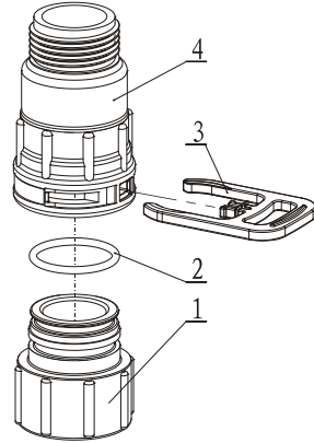
5457002 Animated Connector
