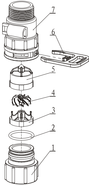
5447018 Flow Meter
